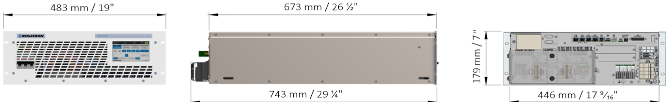
Figure 3: Front, right hand side and rear view. 19-inch module with 4 units in height. Add 83 mm / 3 1/4" to case depth for DC cover or 184 mm / 7 3/8" for DC+AC cover.
