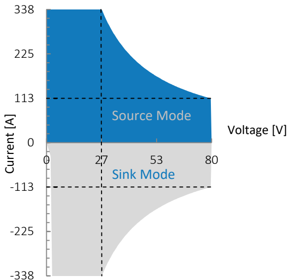
Figure 1: G5.RSS.9.80.338, voltage / current operating area.
